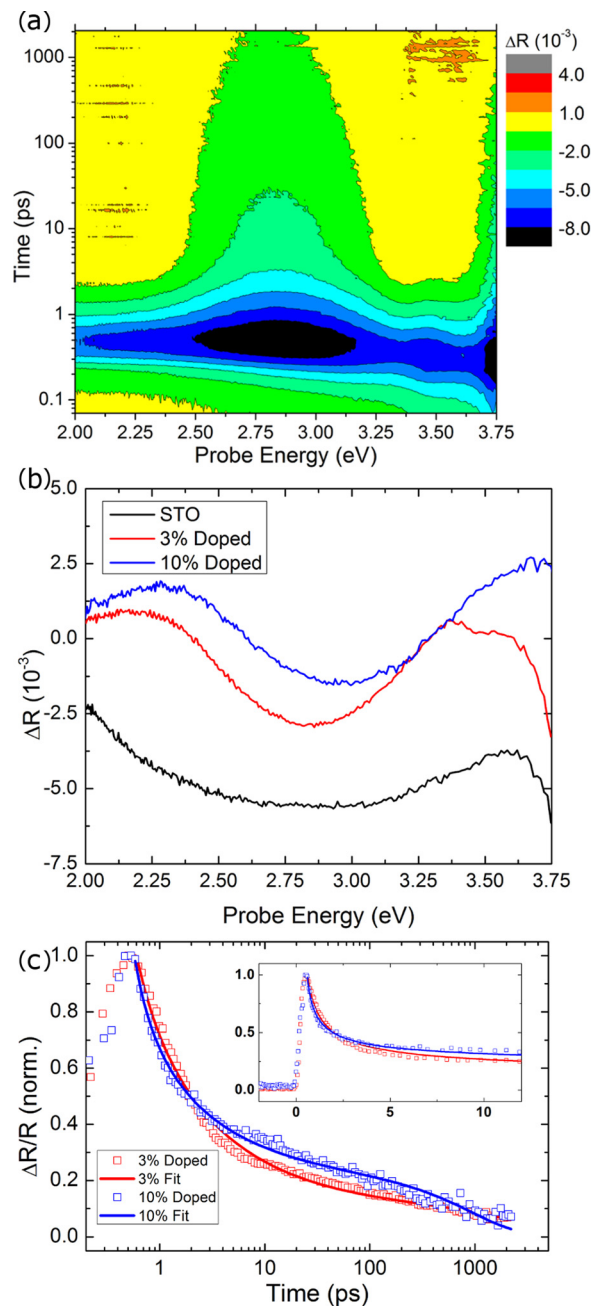
FIG. 2. (a) Map of reflectivity change with time and probe energy; (b) Spectral response at \sim 5 ps; (c) Normalized transient reflectivity at energy corresponding to the minimum \Delta R and model fit. All films were pumped at 4 eV with 1.06 \pm 0.04 mJ/cm 2 pulse.
