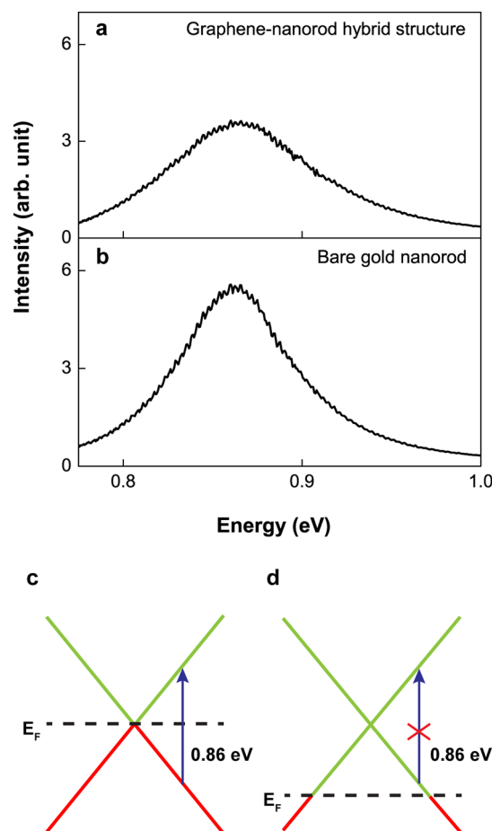
Figure 2. Effect of graphene on the gold nanorod plasmon resonance. (a) Rayleigh scattering spectra of an as-prepared graphene–nanorod hybrid structure. (b) Rayleigh scattering spectrum of a bare gold nanorod. Both scattering spectra exhibit prominent plasmon resonances at 0.86 eV (i.e., at the telecom wavelength of 1.5 \mu\text{m} ), but the resonance in graphene–nanorod hybrid structure is significantly broader due to extra dissipation channel from graphene absorption. (c) Illustration of strong interband optical transitions present at all energies in pristine graphene. They contribute to the plasmon dissipation at 0.86 eV. (d) Illustration showing that a gate-induced shift in Fermi energy ( E_F ) can block the interband transition in graphene and reduce optical dissipation at 0.86 eV.
