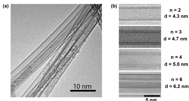
Figure 4. High-resolution TEM images of BNNTs produced by EPIC synthesis. (a) A bundle of double-wall BNNTs; (b) individual BNNTs with different number of walls indicated by n and outer tube diameter indicated by d . High crystallinity is apparent. Under these synthesis conditions 70% of the BNNTs are double wall, n = 2 . Synthesis conditions: same as for Figure 3.
