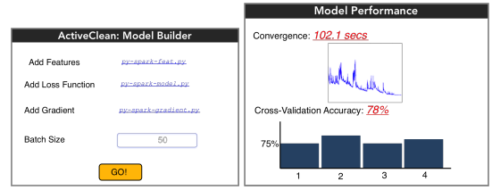
Figure 2: Initialization. The analyst loads user-defined model functions into ActiveClean and then trains an initial model on the dirty data
